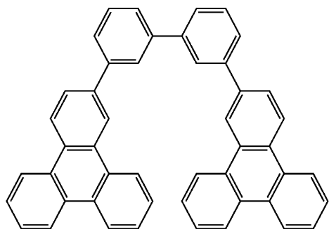
Compound 2
